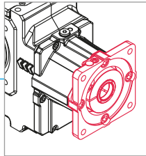
SERVO-Adapter
